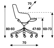
5-legged swiveling height adjustable
