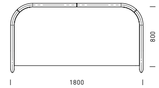
WP-C1800
