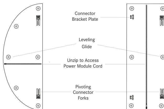
Underside View of Connecting Module Tables
