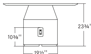
JS2X - 42" Square Power + USB (2)
