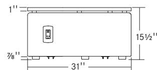
J33X - Single Sided 90° Curved Connecting Table Side View Power + USB (1)
