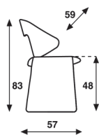
chair without castors
