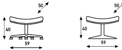
P 141: footstool 5-legged not swiveling
