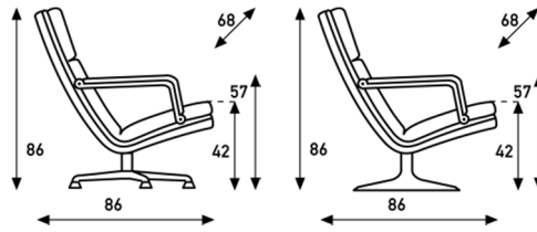
F 141: chair 5-legged swiveling
