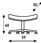
P 141: footstool 5-legged not swiveling
