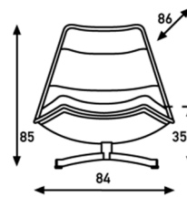
F 586 L: chair low swiveling
