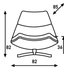
F 512 L: chair low swiveling
